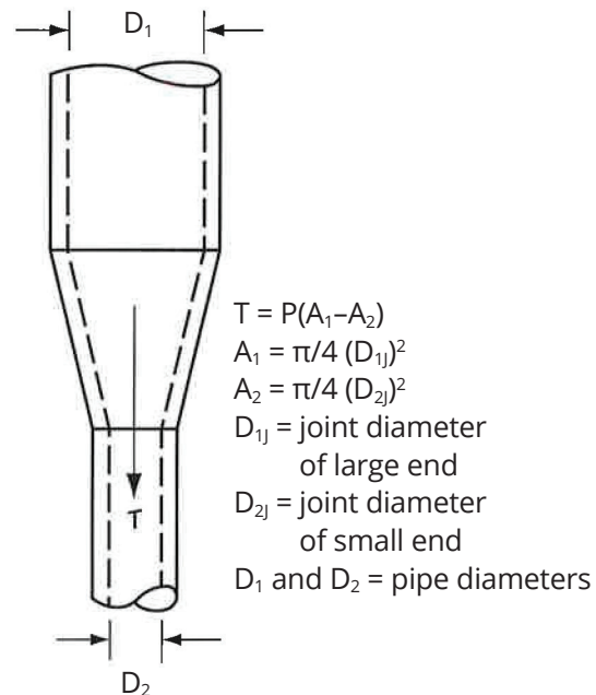
Figure 13-3D - Reducer thrust
