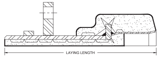
ANCHORED MECHANICAL JOINT BELL X BELL
