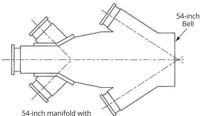
54-inch manifold with five 20-inch flange branches
