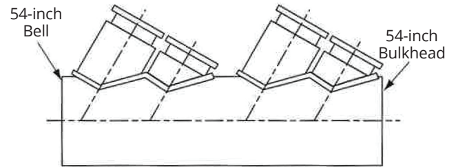
54-inch manifold with four 30-inch flange outlets
