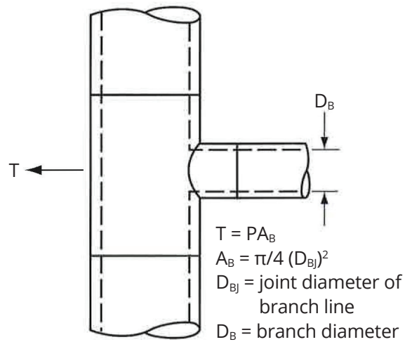
Figure 13-3C - Tee thrust
