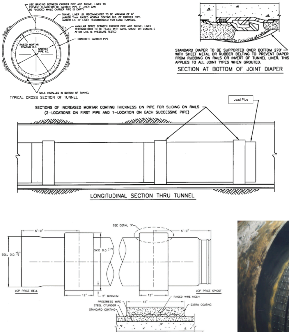
Figure 3: Approximate dimensions of raised mortar coating skids.
