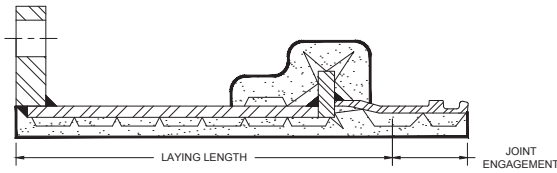
BELL x FLANGE ADAPTER
