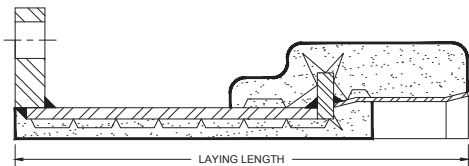
BELL x FLANGE ADAPTER
