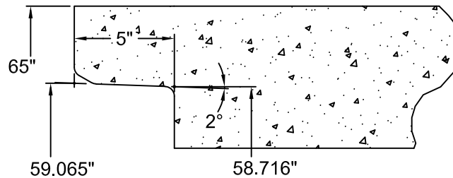
BELL END
