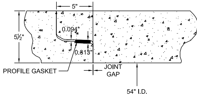
JOINT ASSEMBLY
